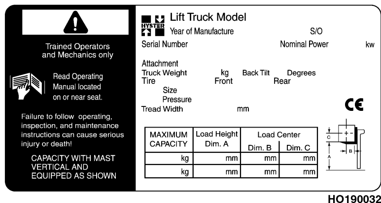
Figure 11. Plaque d'identification
