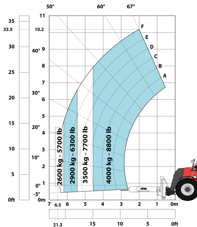
Machine on tyres with cylinder handler CH 4 (Metric)
