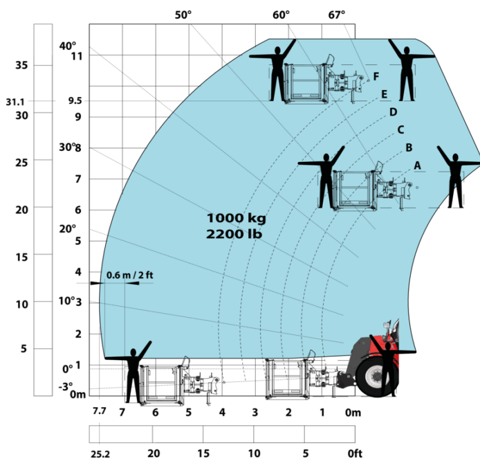
Machine on tyres with platform Metric
