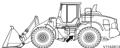
Positie vetreservoir
