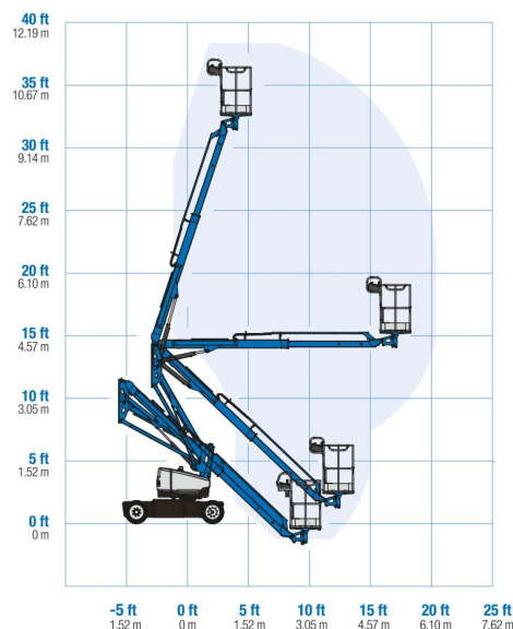
Range Of Motion Z-33/18
